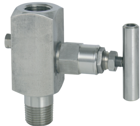
Barstock single block valve, form 2, male/female ½ NPT, PN 420, DN 5
