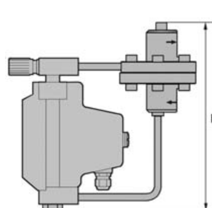
DK37/M8E with outlet pressure regulator
