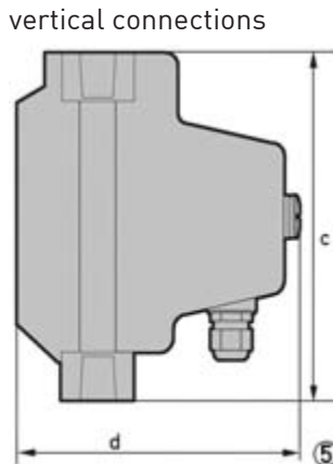
DK37/M8E without valve and vertical connections
