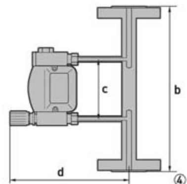
DK32 with flange connections
